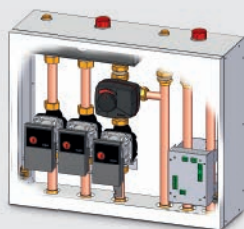
Kit Hydraulique BIO DMS
