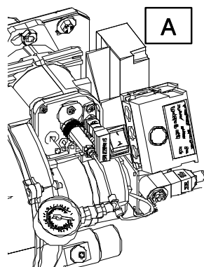
DANFOSS – MOD. BFP 21 L3 071N2132
